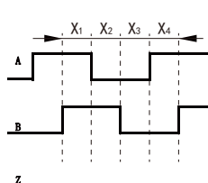
Waveform for C, E, F output
